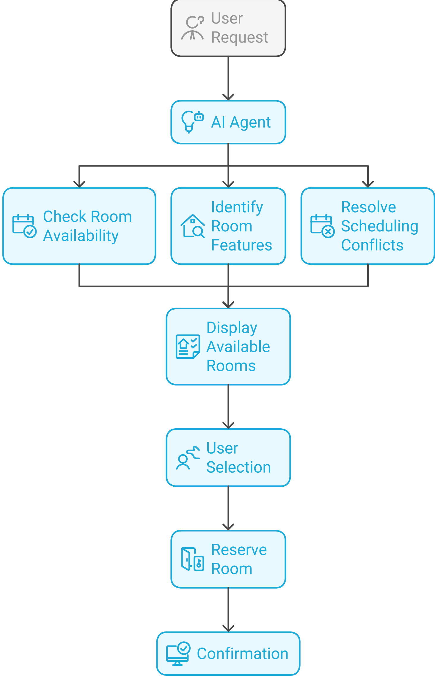
LangGraph-based AI Agent for Meeting Room Management
