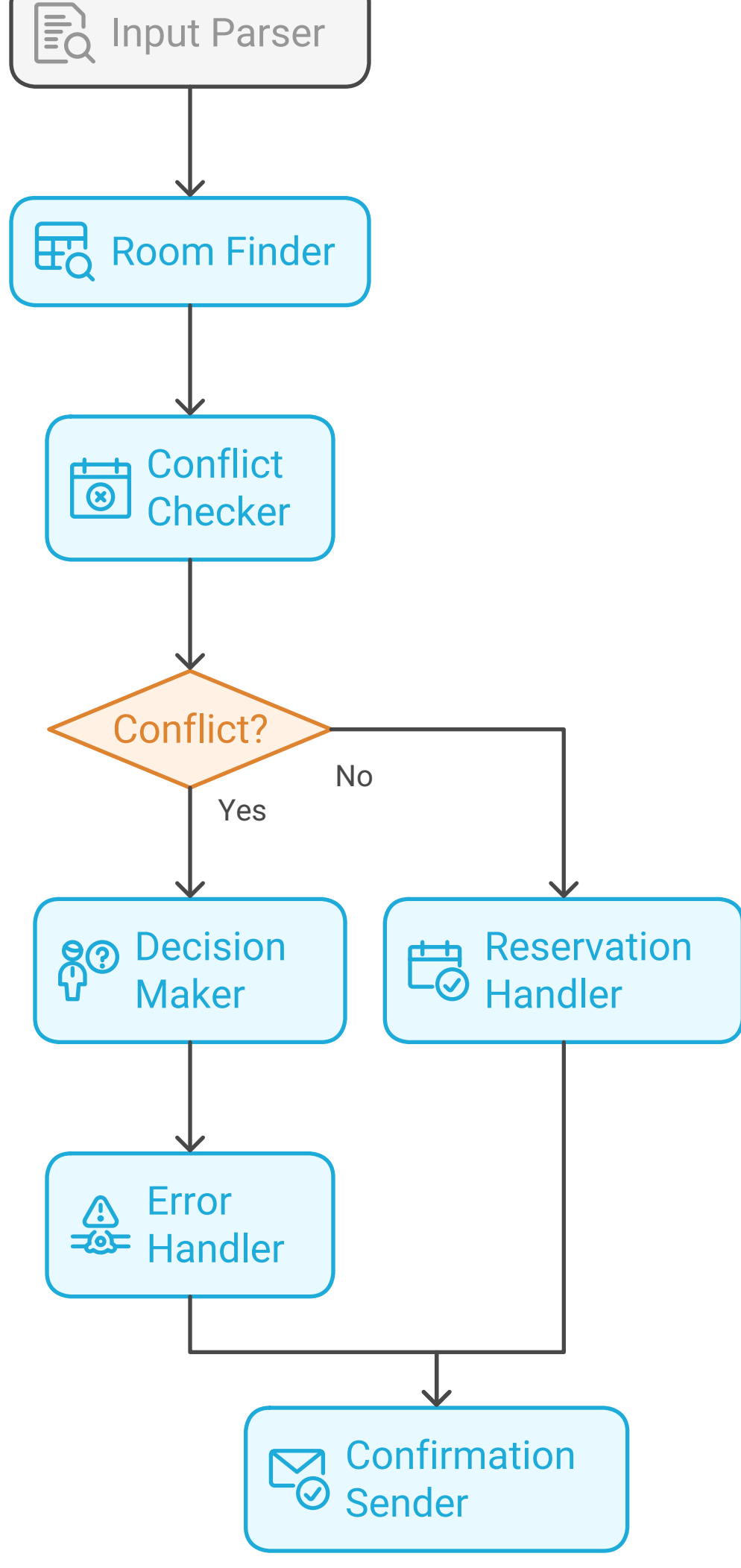
Room Booking Process Flowchart
